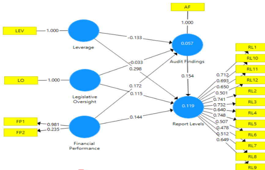
1 Figure 2 – Initial PLS Algorithm Results
